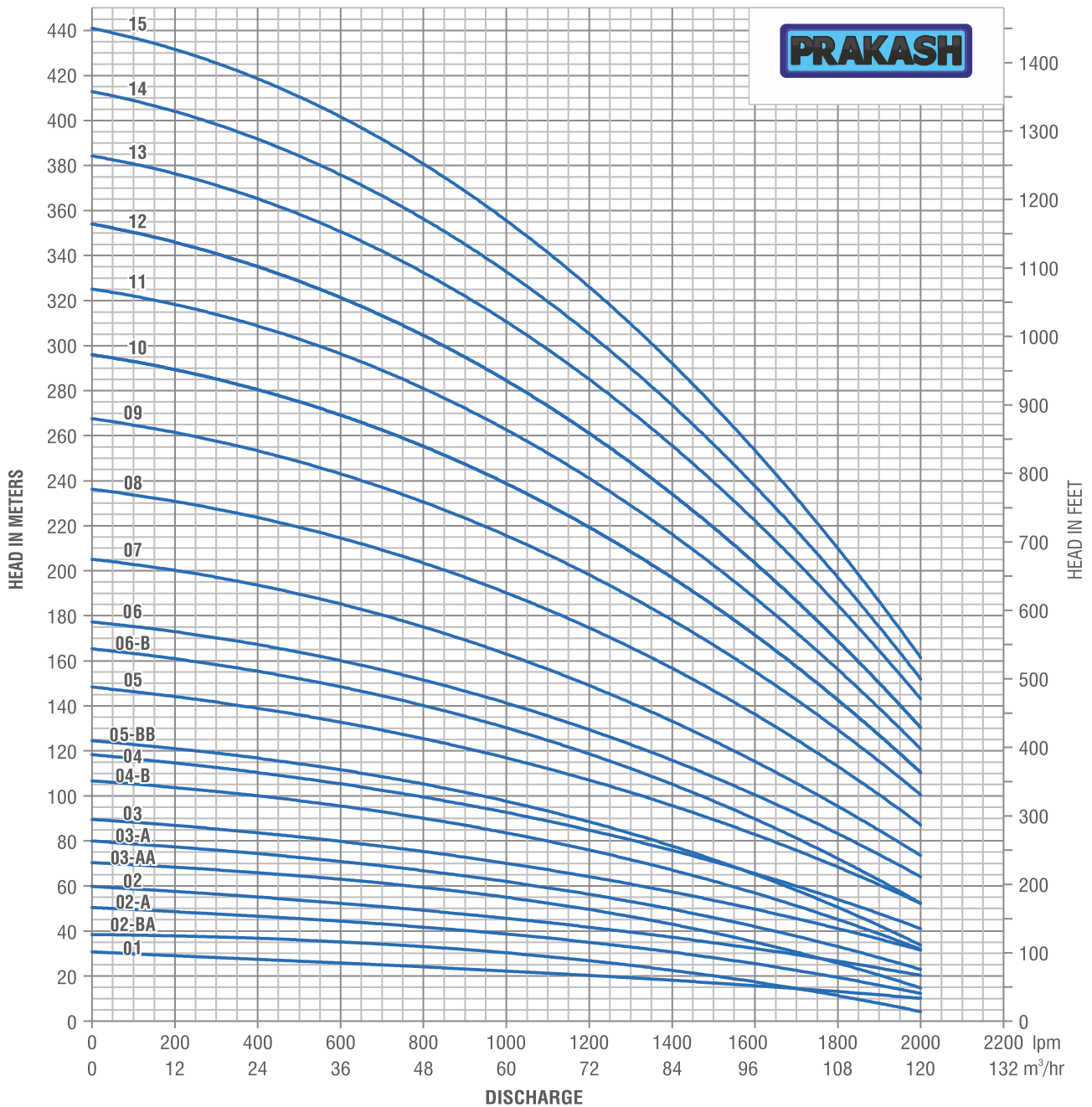
HYDRAULIC PERFORMANCE CURVE SP-M77A, 60Hz, 3450rpm
