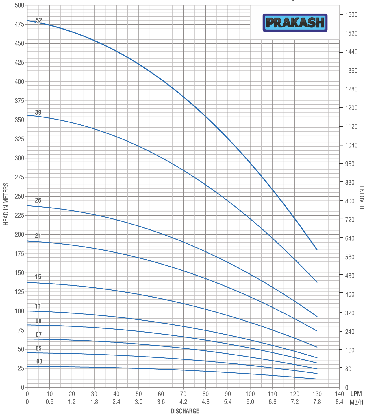
HYDRAULIC PERFORMANCE CURVE SP-R5A, 60Hz, 3450 rpm
