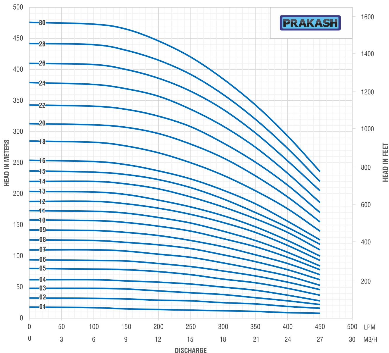
HYDRAULIC PERFORMANCE CURVE SP-R17A 3450 rpm , 60Hz
