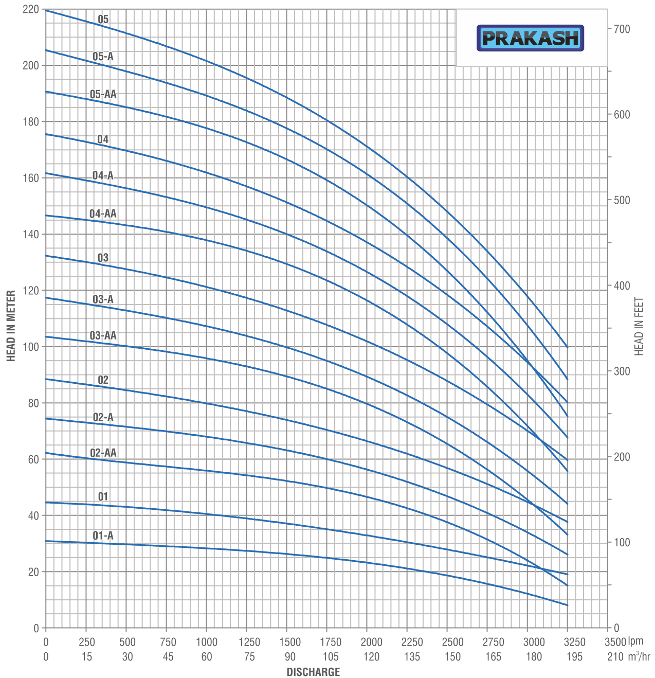
HYDRAULIC PERFORMANCE CURVE SP-M125A 60Hz, 3450 rpm
