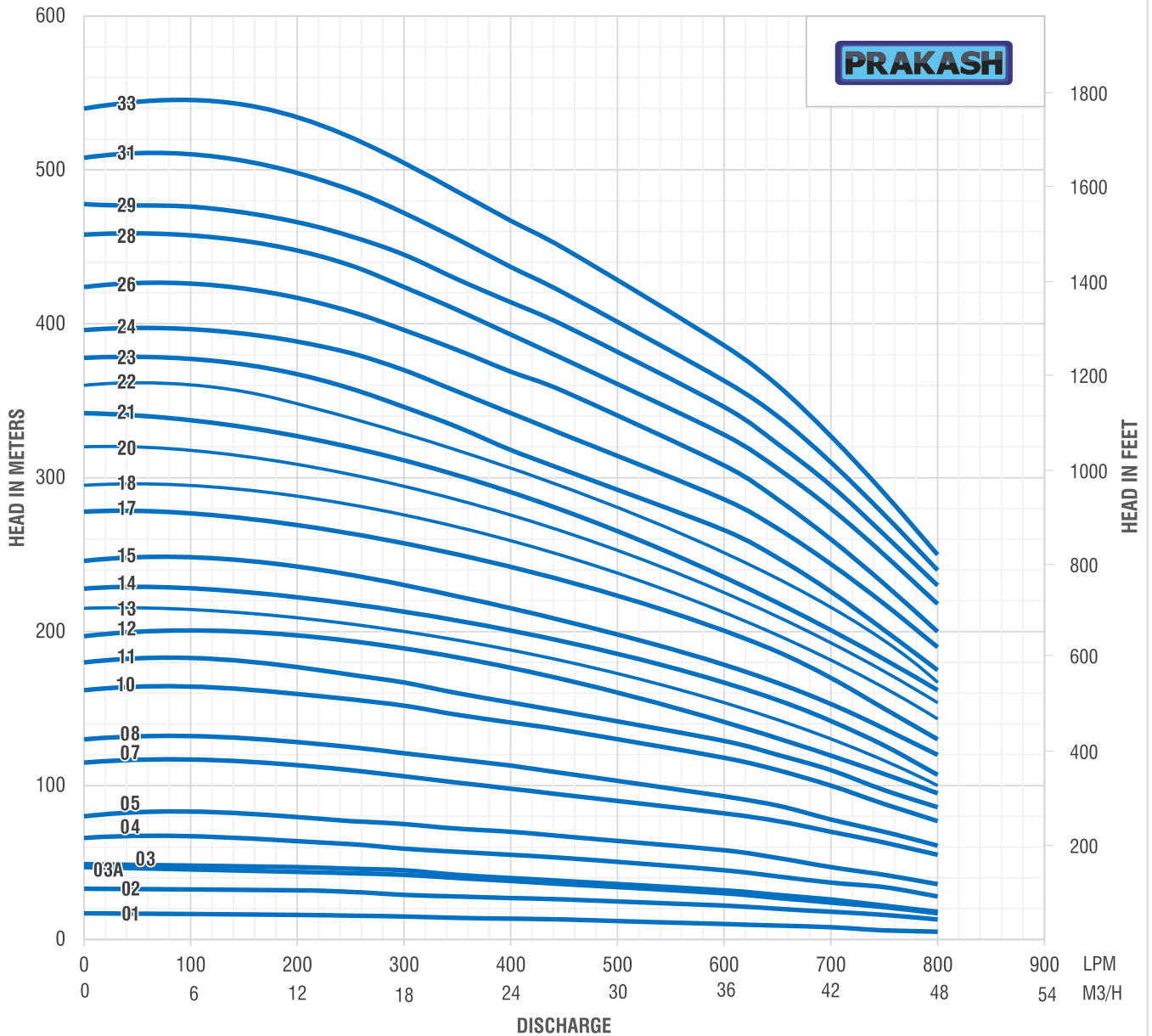
HYDRAULIC PERFORMANCE CURVE SP-M30A 3450RPM, 60Hz
