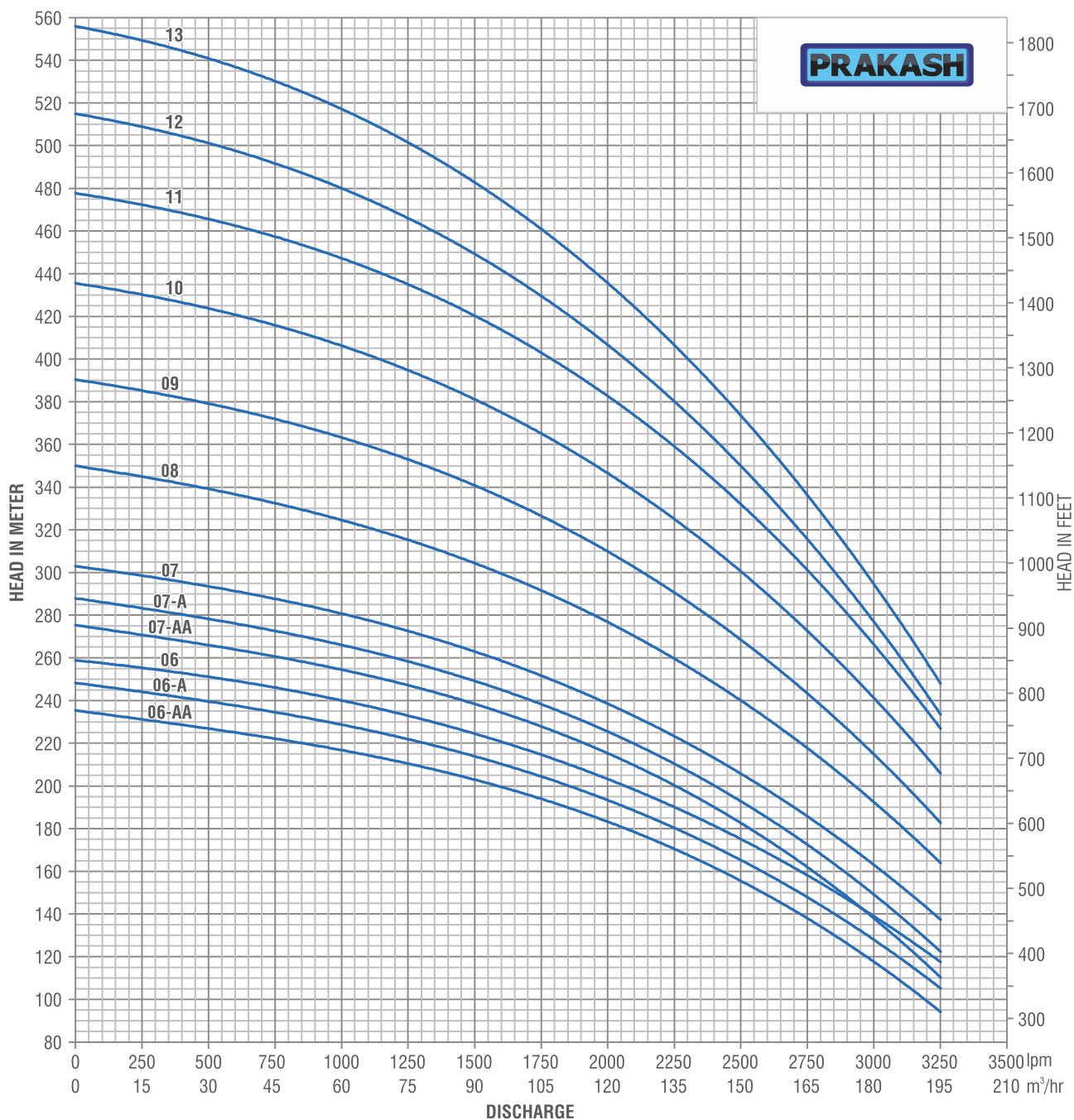
HYDRAULIC PERFORMANCE CURVE SP-M125A 60Hz, 3450 rpm
