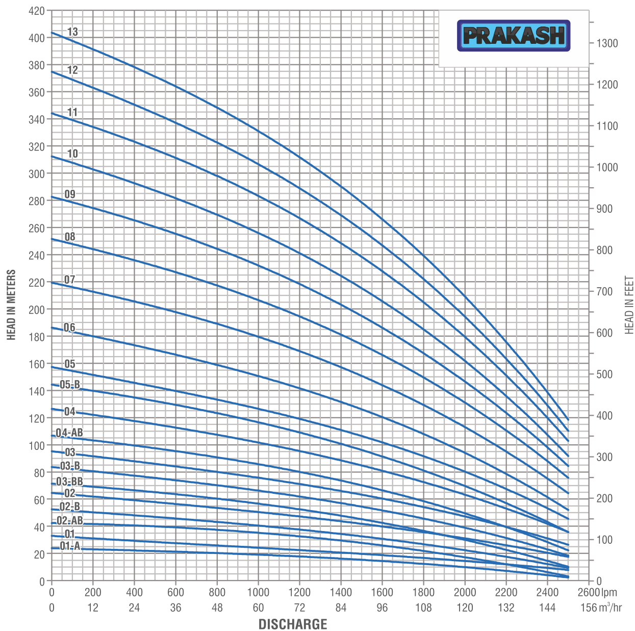
HYDRAULIC PERFORMANCE CURVE SP-M95A, 60Hz, 3450rpm
