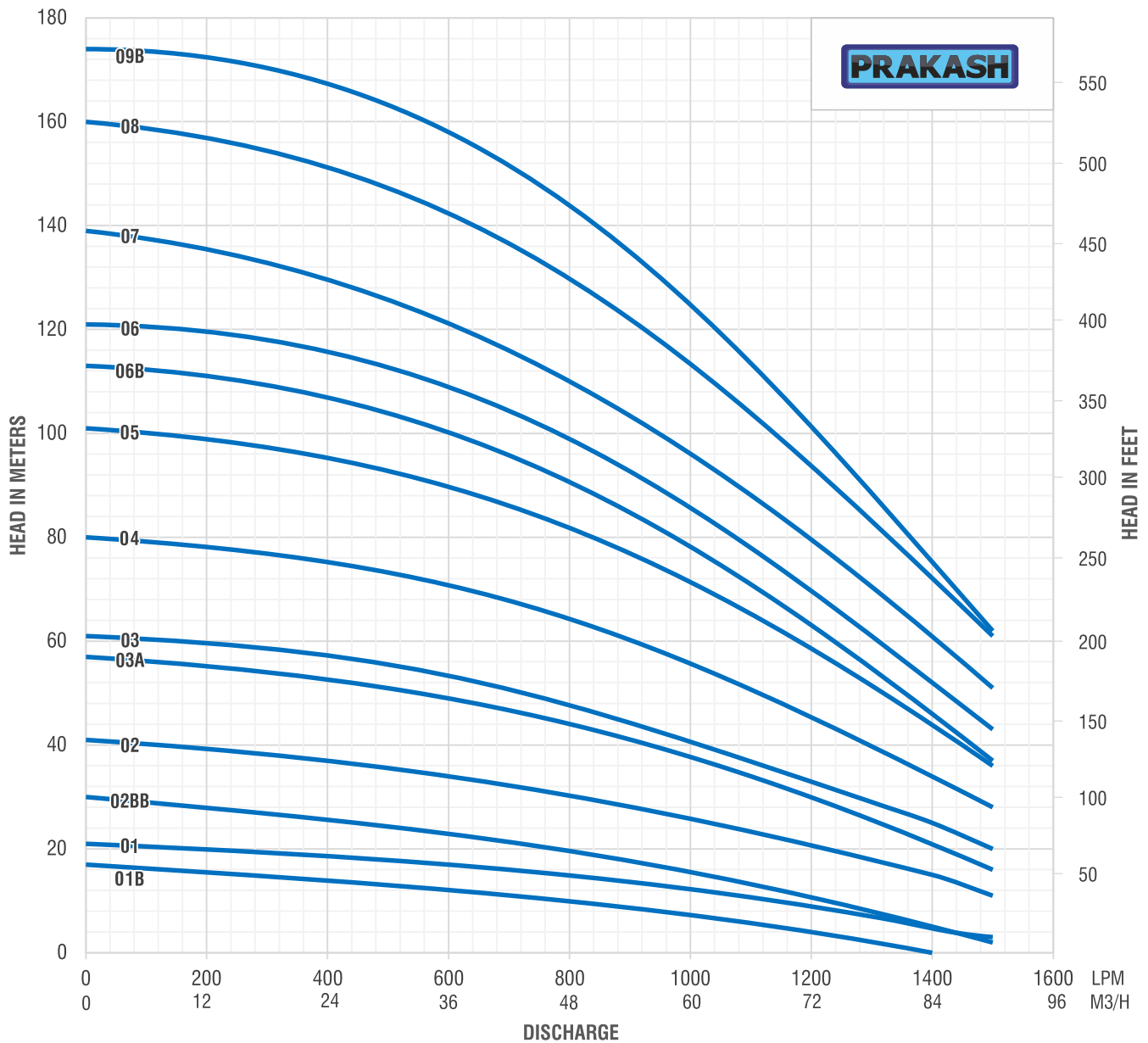
HYDRAULIC PERFORMANCE CURVE SP-M60A 3450RPM, 60Hz
