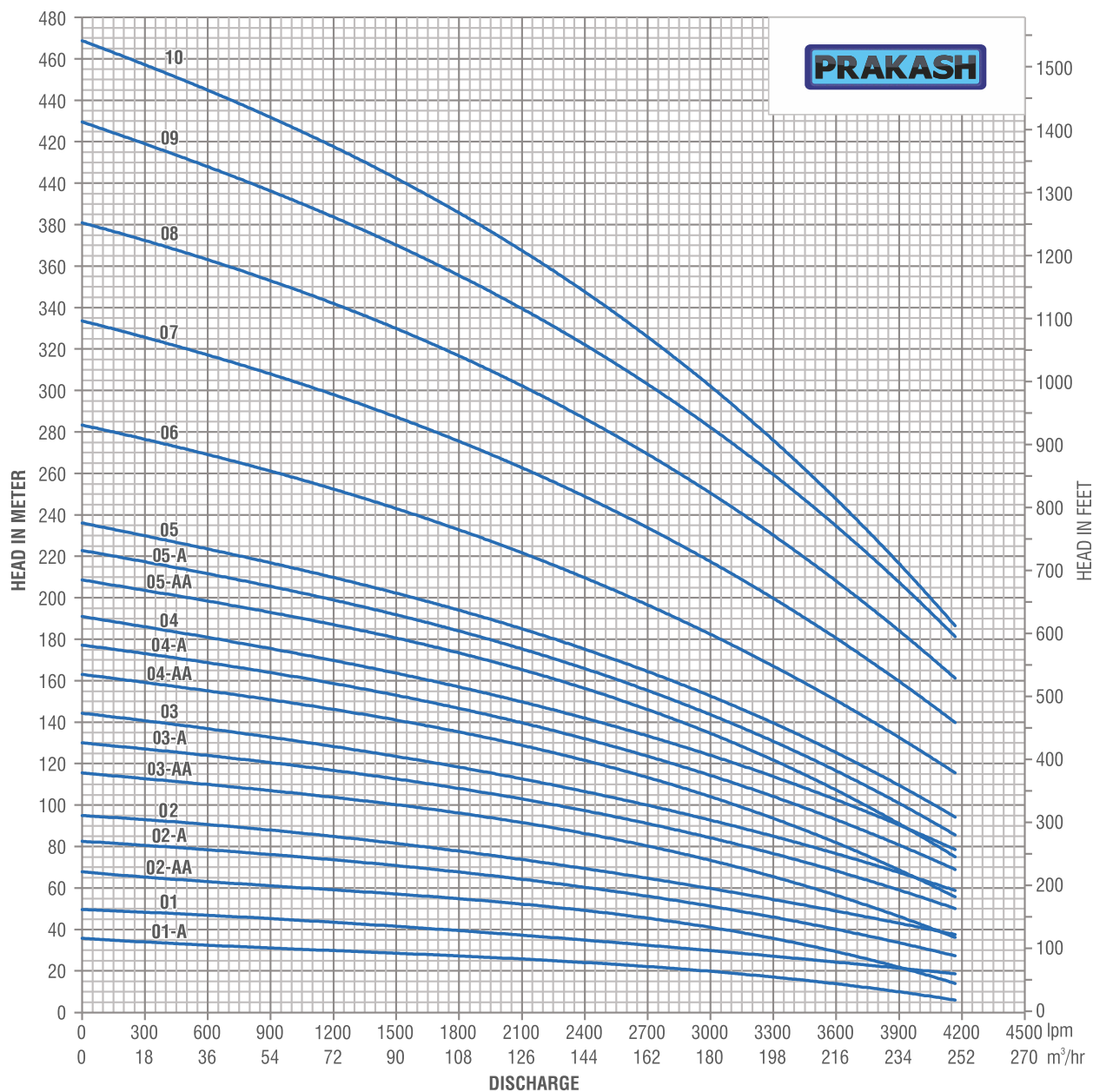
HYDRAULIC PERFORMANCE CURVE SP-M160A 60Hz, 3450 rpm
