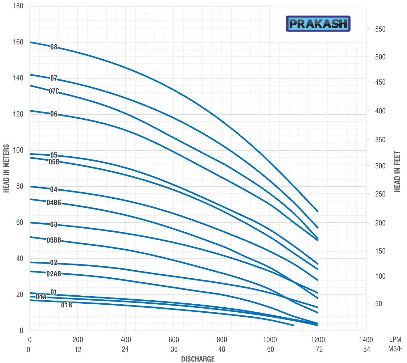
HYDRAULIC PERFORMANCE CURVE SP-M46A 3450RPM, 60Hz
