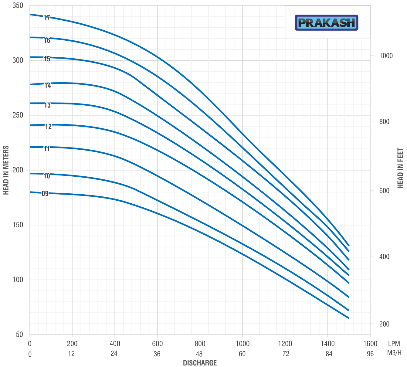
HYDRAULIC PERFORMANCE CURVE SP-M60A 3450RPM, 60Hz
