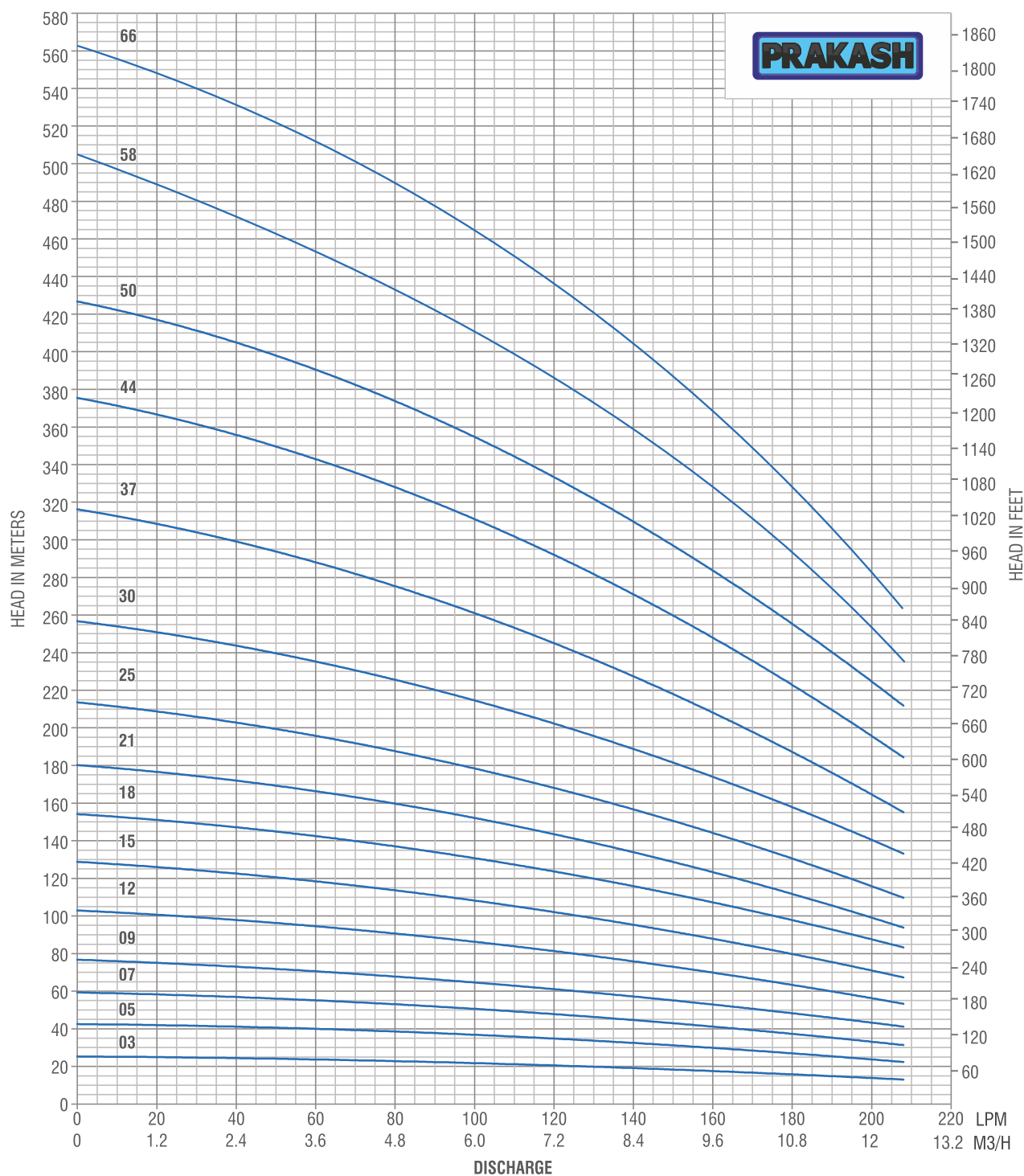
HYDRAULIC PERFORMANCE CURVE SP-R8A, 60Hz, 3450 rpm
