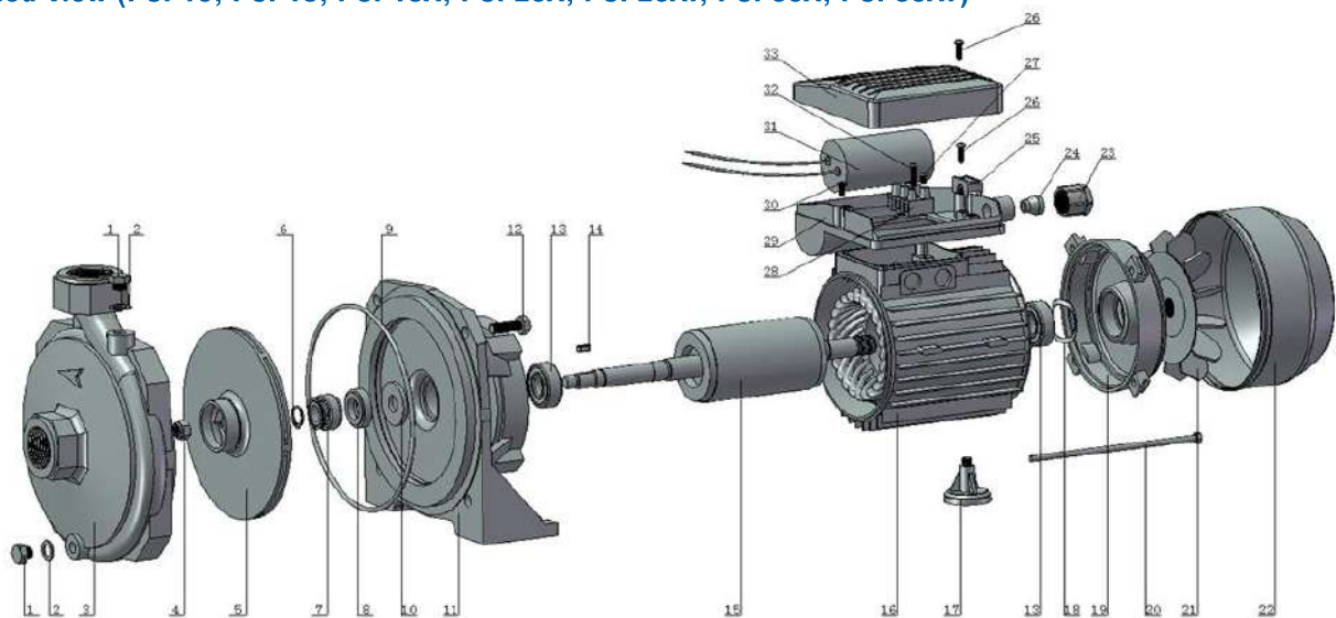
Exploded view (PCP10, PCP15, PCP15A, PCP20A, PCP20AT, PCP30A, PCP30AT)
