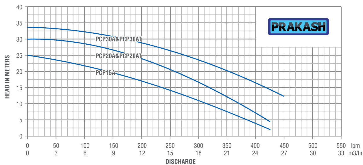
HYDRAULIC PERFORMANCE CURVE PCP15A, 20A, 20AT, 30A, 30AT, 50Hz, 2900RPM
