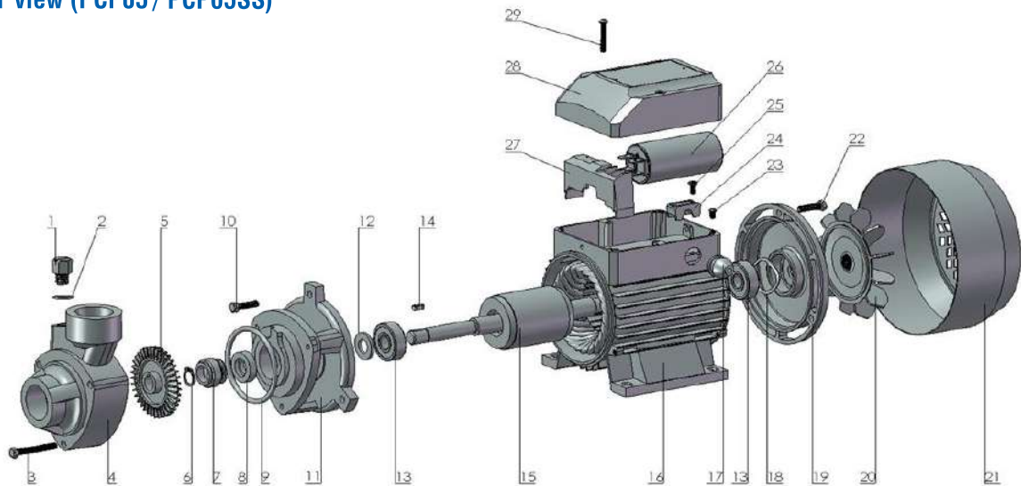
Exploded view (PCP05 / PCP05SS)
