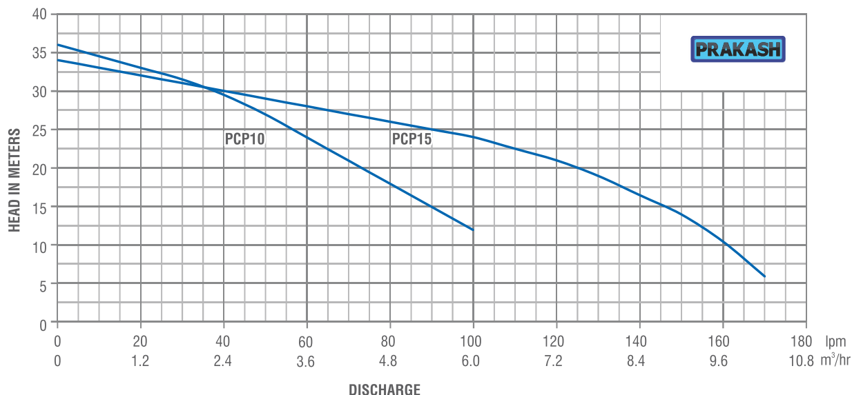
HYDRAULIC PERFORMANCE CURVE PCP10, PCP15, 60Hz, 3500 RPM
