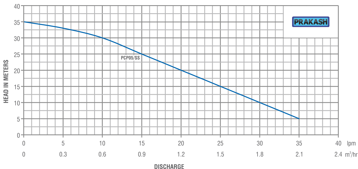
HYDRAULIC PERFORMANCE CURVE PCP05 / PCP05SS, 60Hz, 3500 RPM
