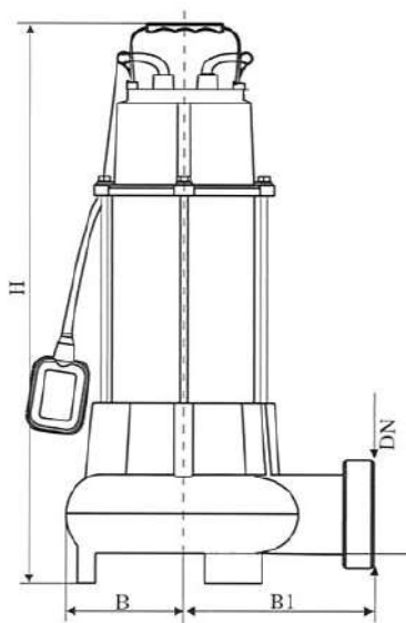
G.A. Drawing
