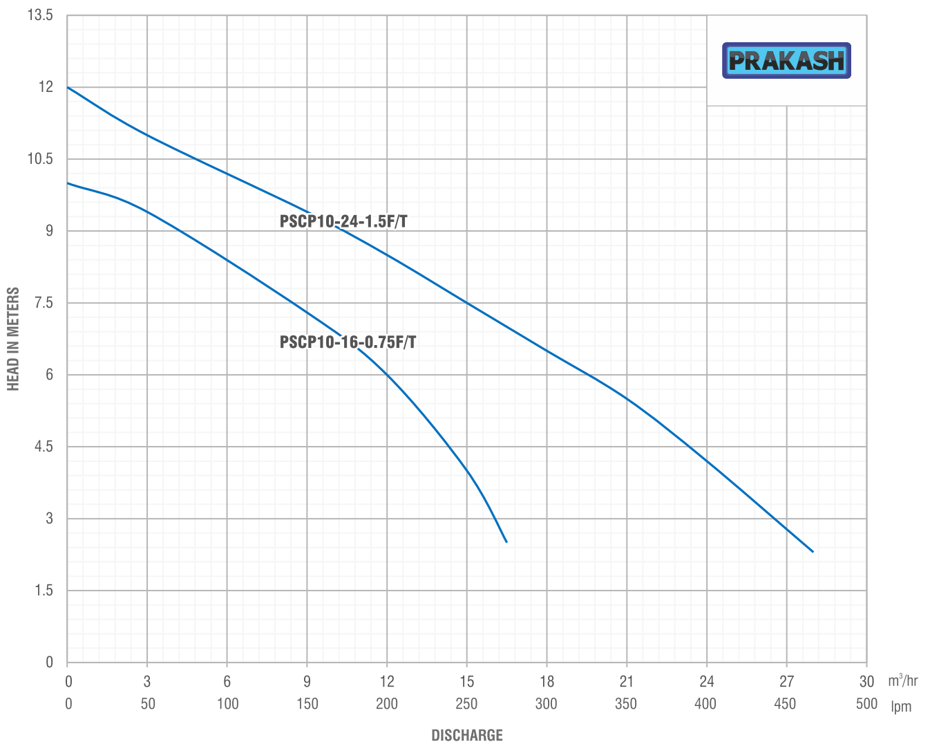
HYDRAULIC PERFORMANCE CURVE PSCP10-16-0.75F/T & PSCP10-24-1.5F/T, 3450RPM, 60HZ
