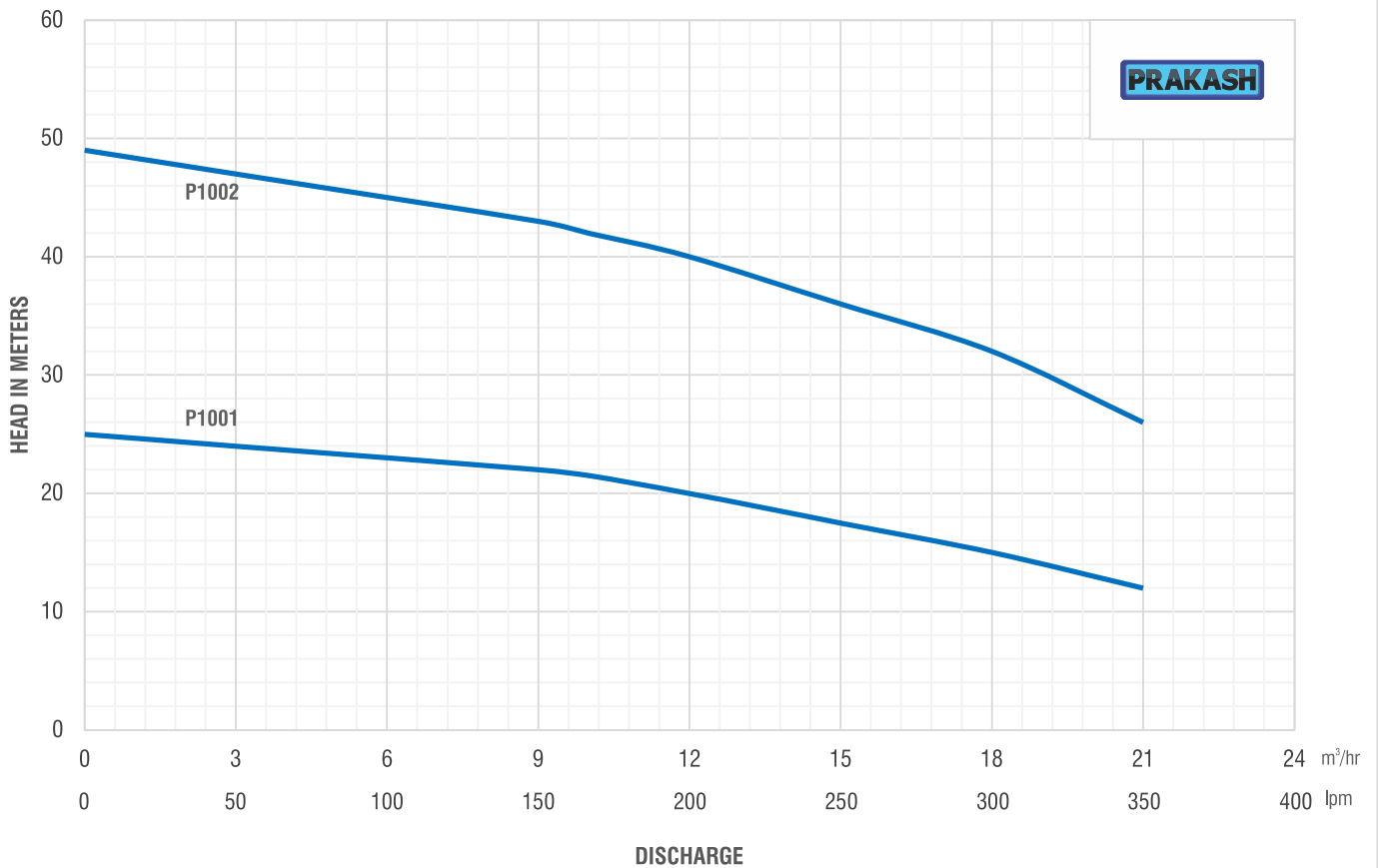
HYDRAULIC PERFORMANCE CURVE P1001 & P1002, 3450RPM, 60Hz
