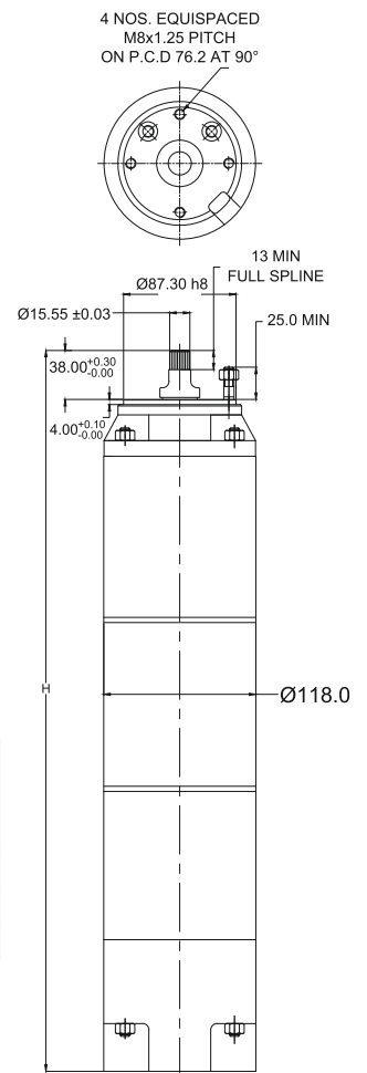
PSMC125 Motor
