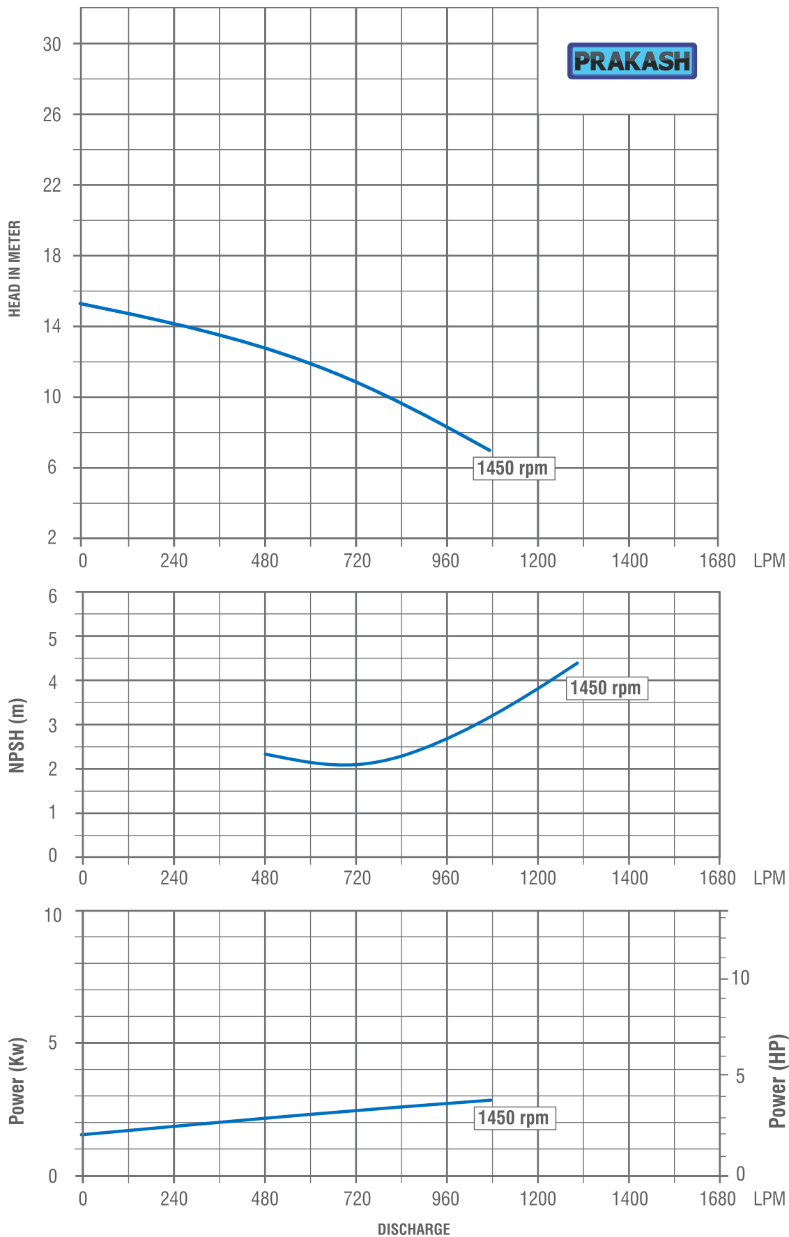
HYDRAULIC PERFORMANCE CURVE PSPSP80-215 1450RPM, 50Hz
