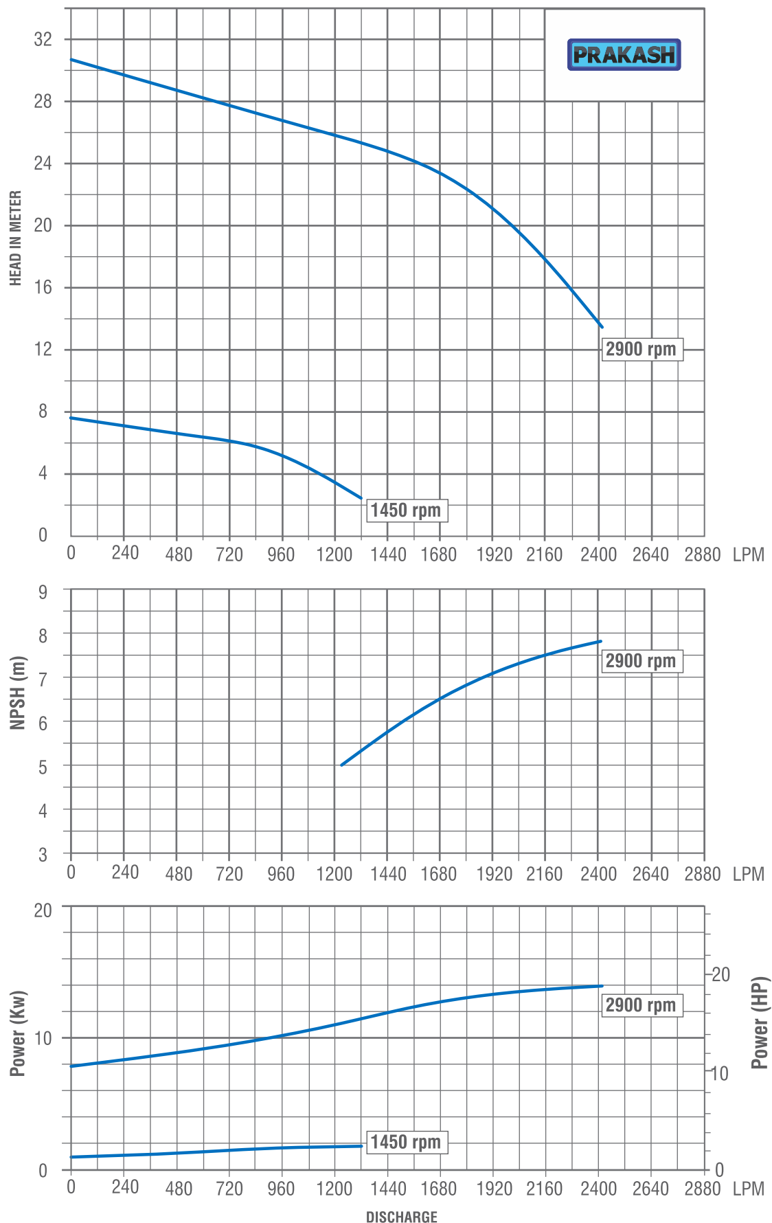
HYDRAULIC PERFORMANCE CURVE PSPSP100-160 1450 & 2900RPM, 50Hz
