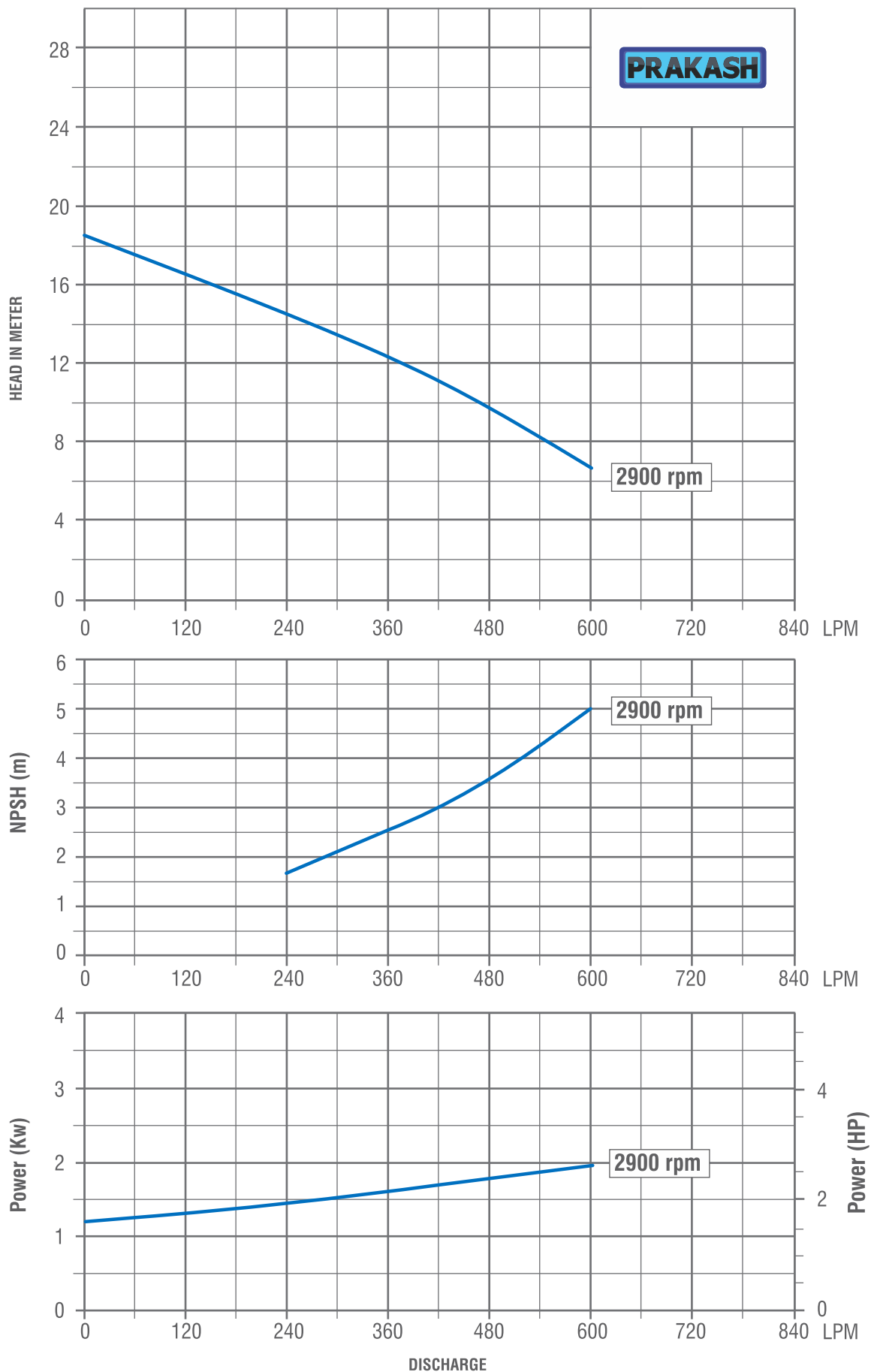
HYDRAULIC PERFORMANCE CURVE PSPSP50-120 2900RPM, 50Hz
