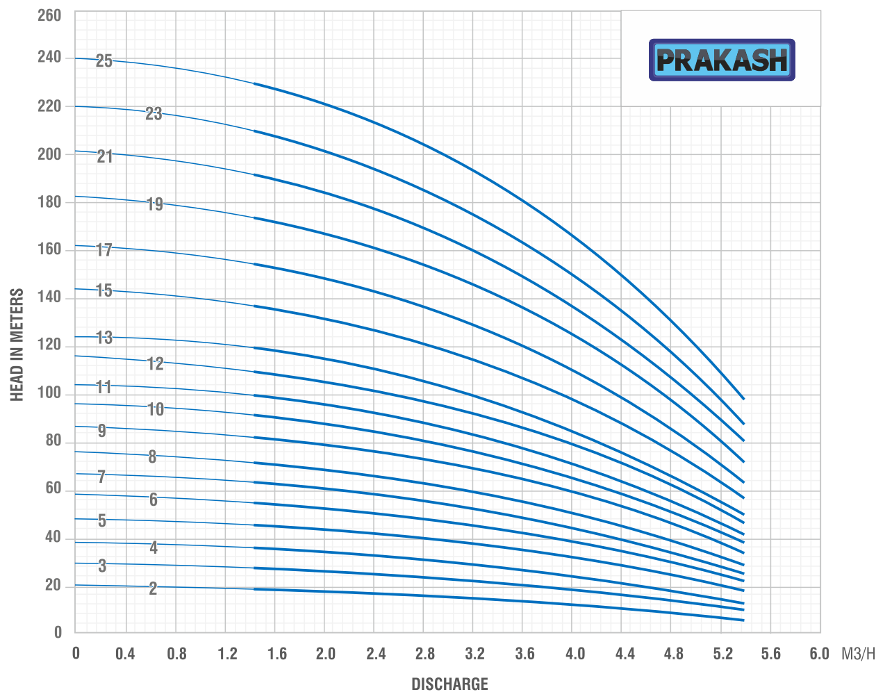
HYDRAULIC PERFORMANCE CURVE PVMP3, 3500RPM, 60Hz
