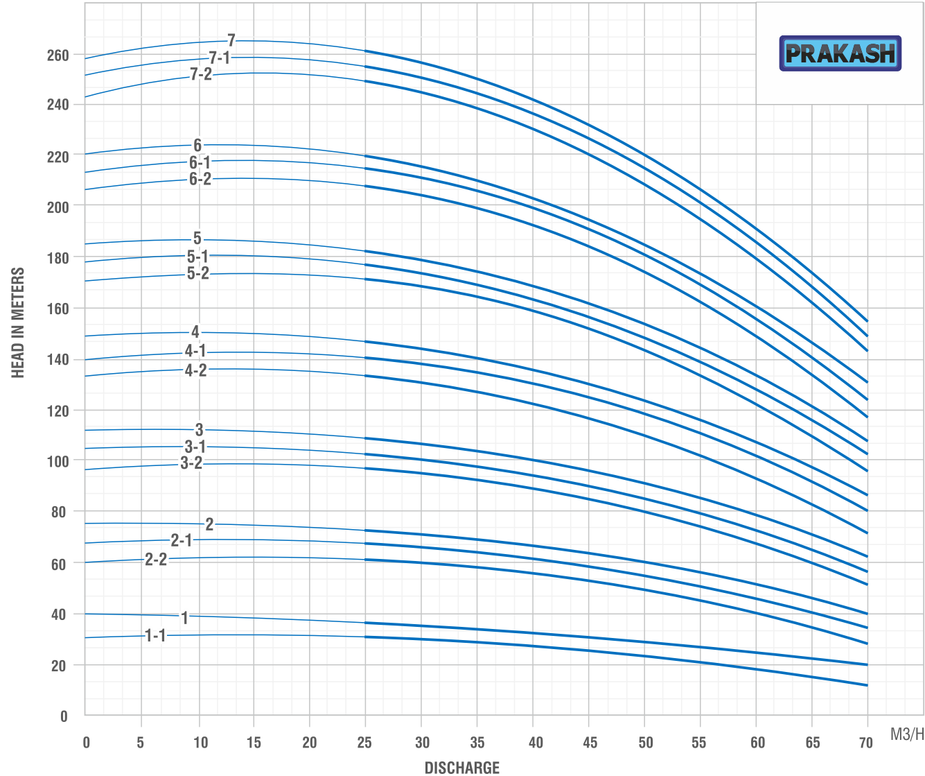
HYDRAULIC PERFORMANCE CURVE PVMP45, 3500RPM, 60Hz
