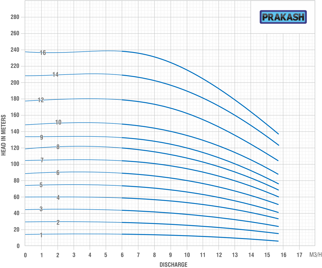
HYDRAULIC PERFORMANCE CURVE PVMP10, 3500RPM, 60Hz
