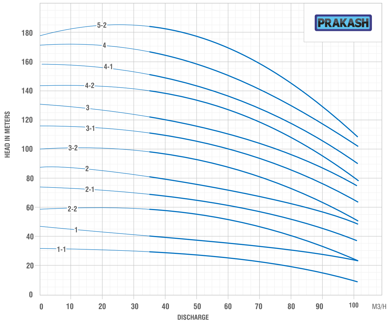
HYDRAULIC PERFORMANCE CURVE PVMP64, 3500RPM, 60Hz
