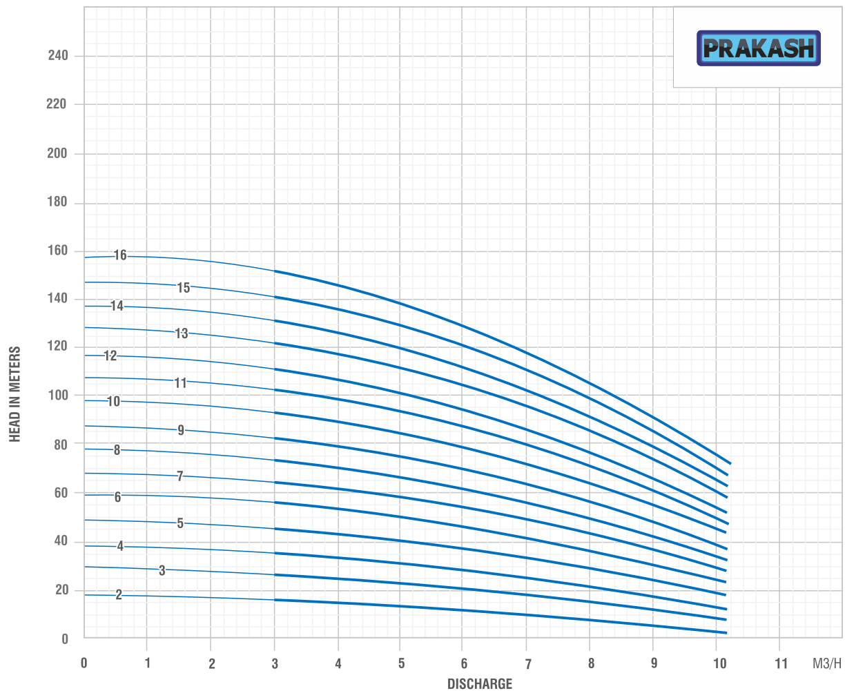
HYDRAULIC PERFORMANCE CURVE PVMP5, 3500RPM, 60Hz
