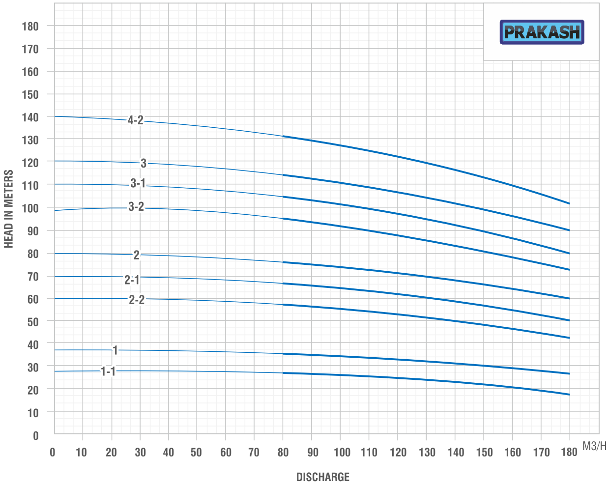
HYDRAULIC PERFORMANCE CURVE PVMP150, 3500RPM, 60Hz
