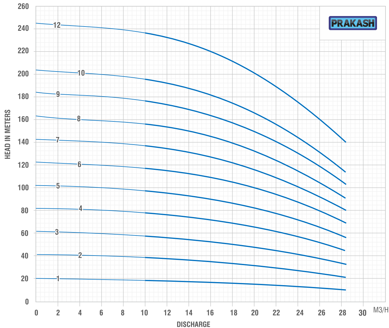
HYDRAULIC PERFORMANCE CURVE PVMP15, 3500RPM, 60Hz
