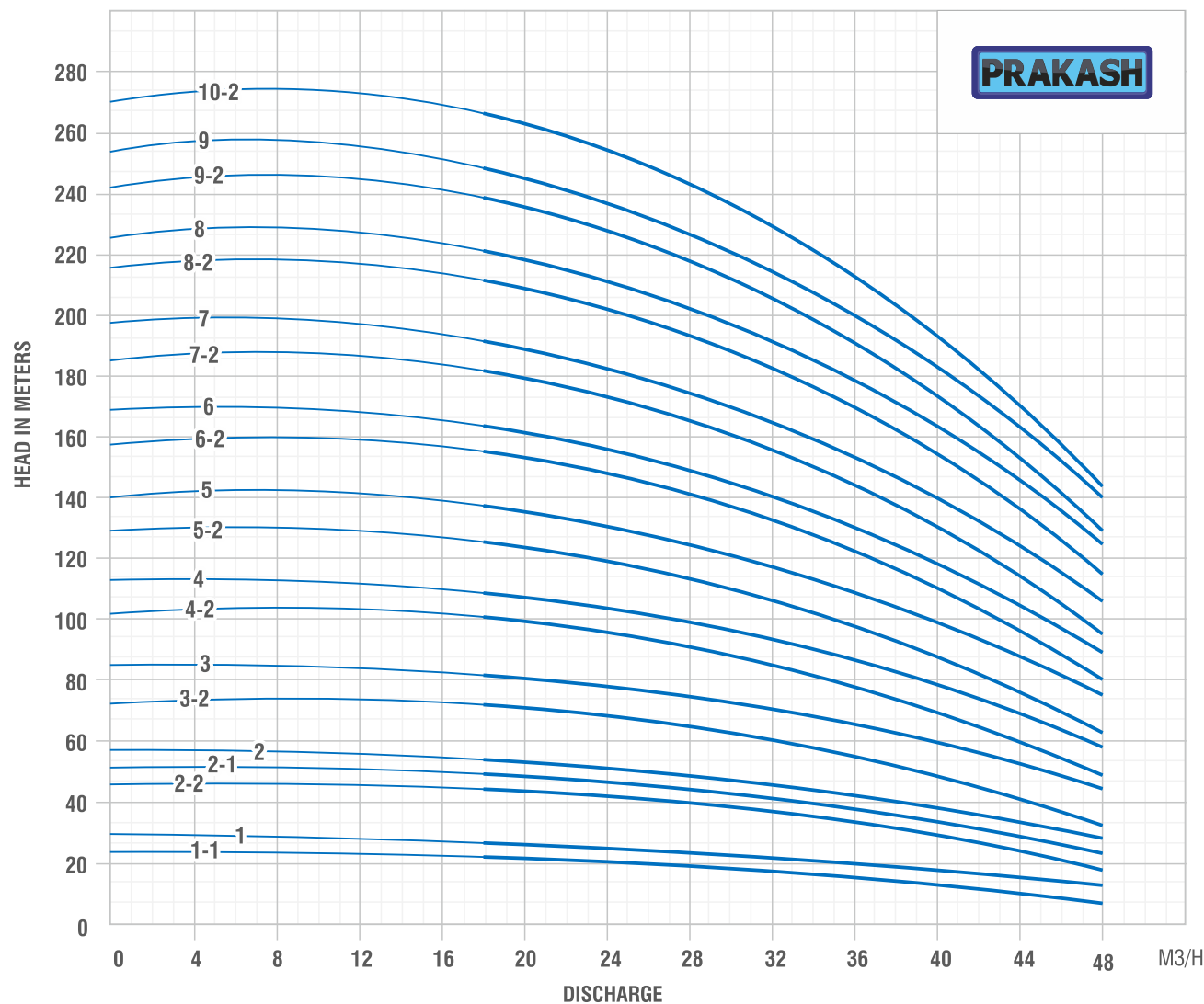
HYDRAULIC PERFORMANCE CURVE PVMP32, 3500RPM, 60Hz
