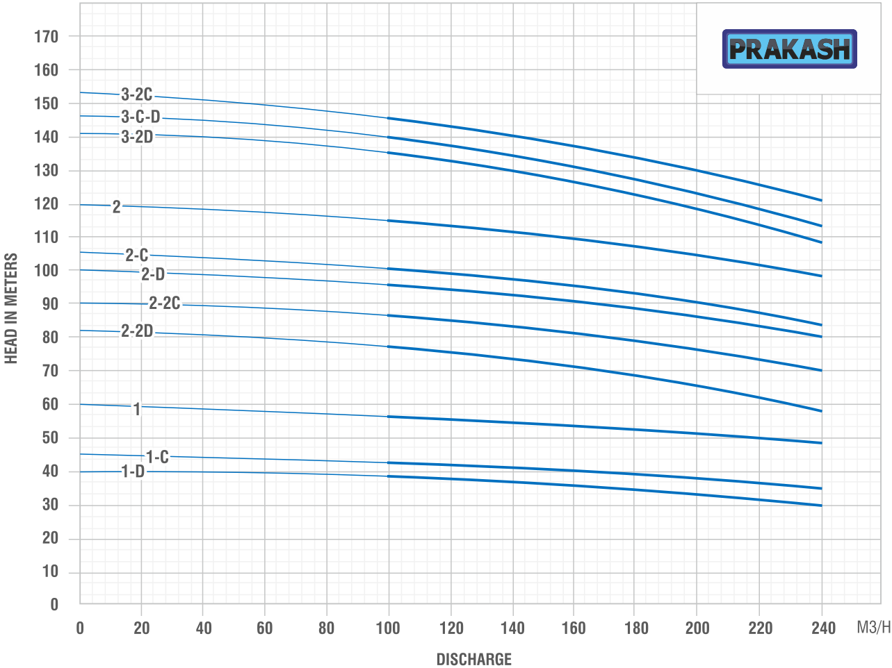
HYDRAULIC PERFORMANCE CURVE PVMP200, 3500RPM, 60Hz
