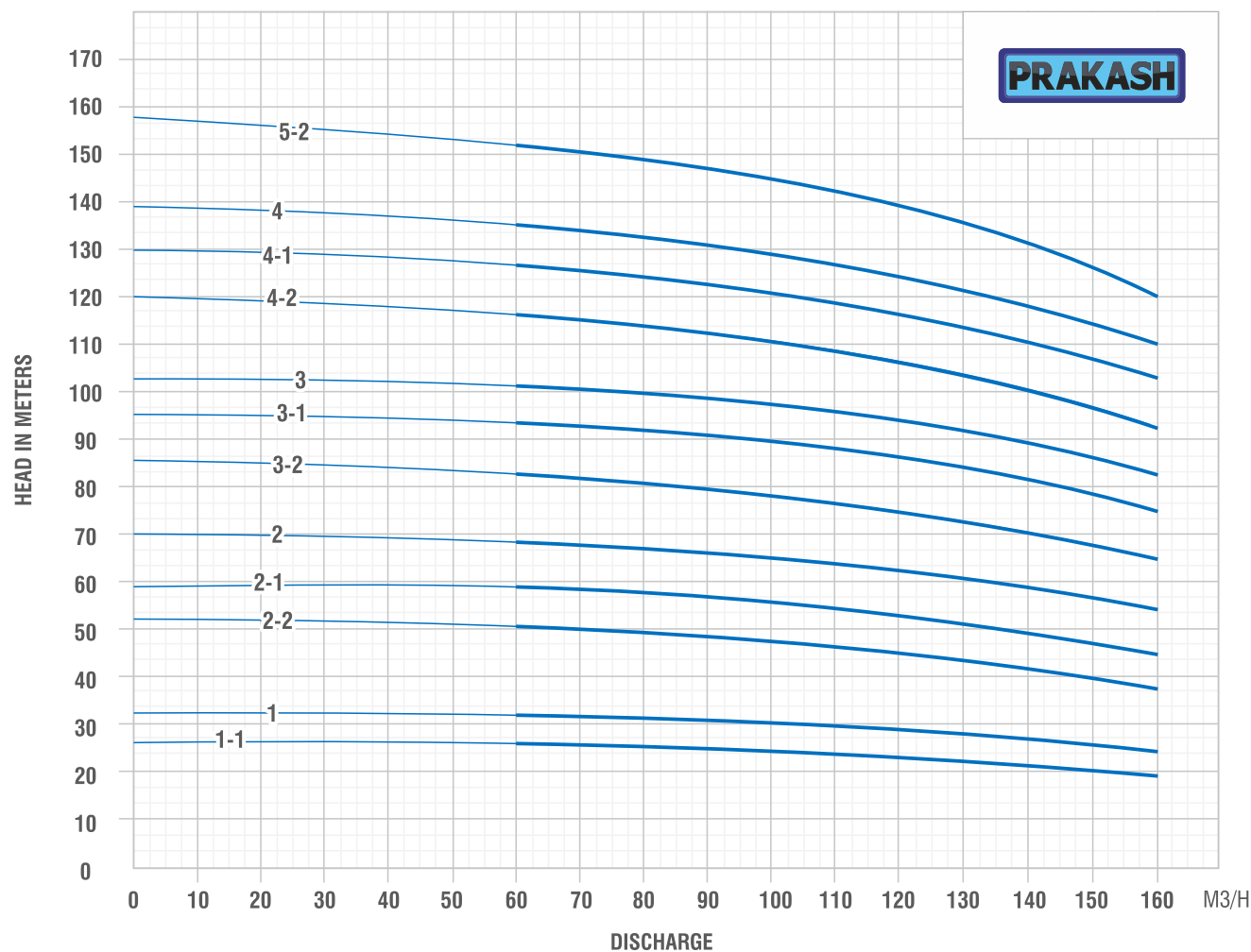
HYDRAULIC PERFORMANCE CURVE PVMP120, 3500RPM, 60Hz
