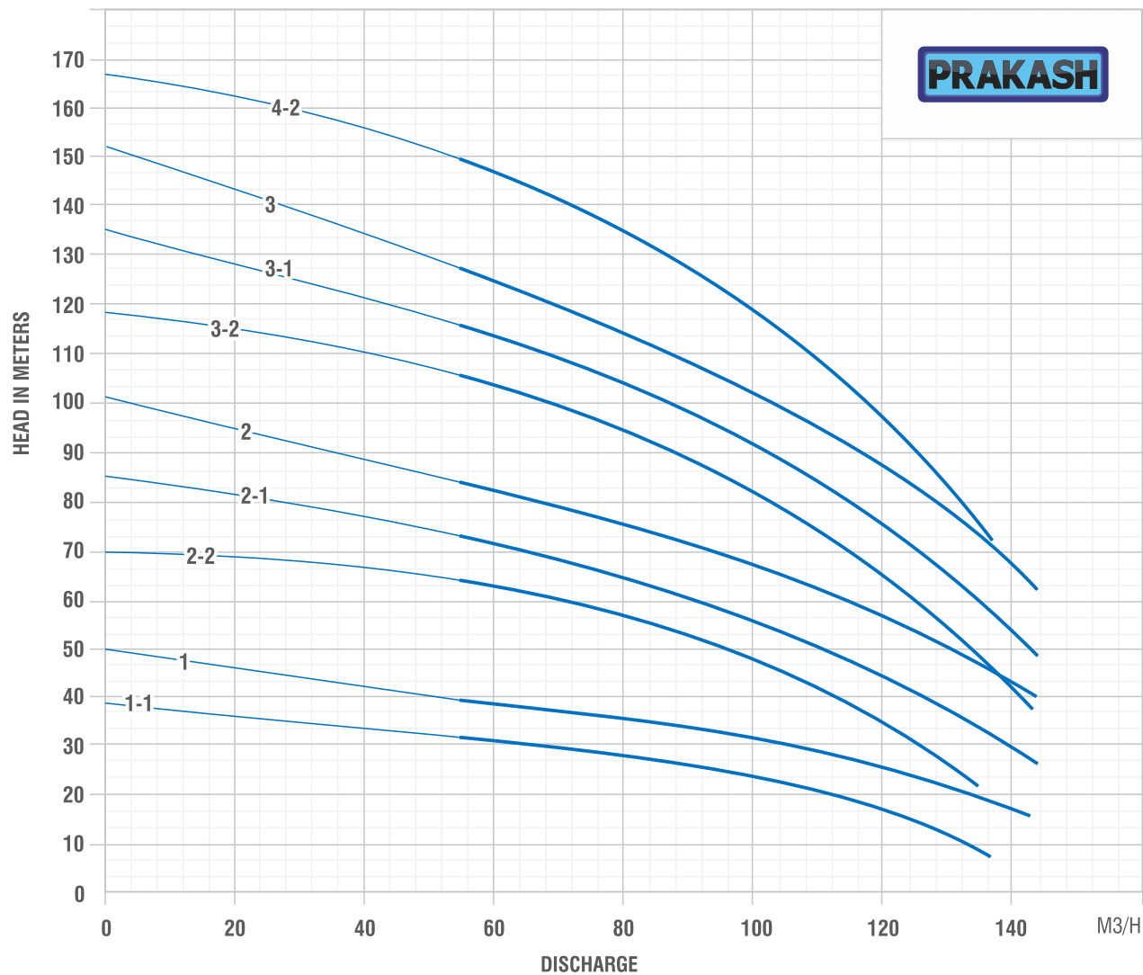
HYDRAULIC PERFORMANCE CURVE PVMP90, 3500RPM, 60Hz
