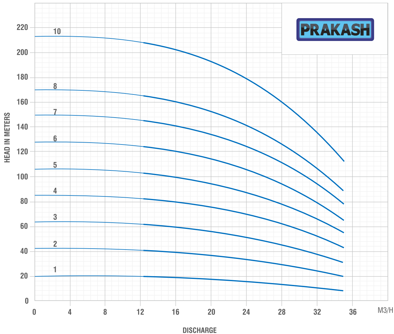
HYDRAULIC PERFORMANCE CURVE PVMP20, 3500RPM, 60Hz
